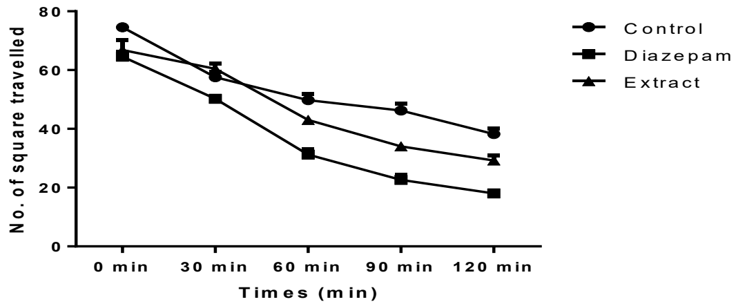
Figure 2: Open field test of methanolic extract of S. villosa , all values are expressed as mean \pm SEM (n = 5); One way Analysis of Variance (ANOVA).
