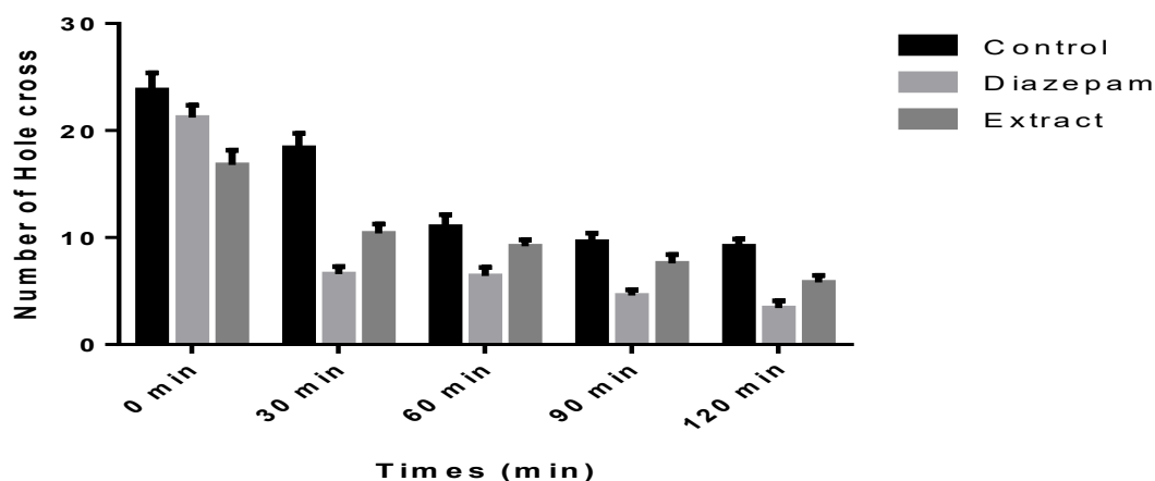
Figure 1: Hole cross test of methanolic extract of S. villosa , all values are expressed as mean ± SEM (n = 5); One way Analysis of Variance (ANOVA).
